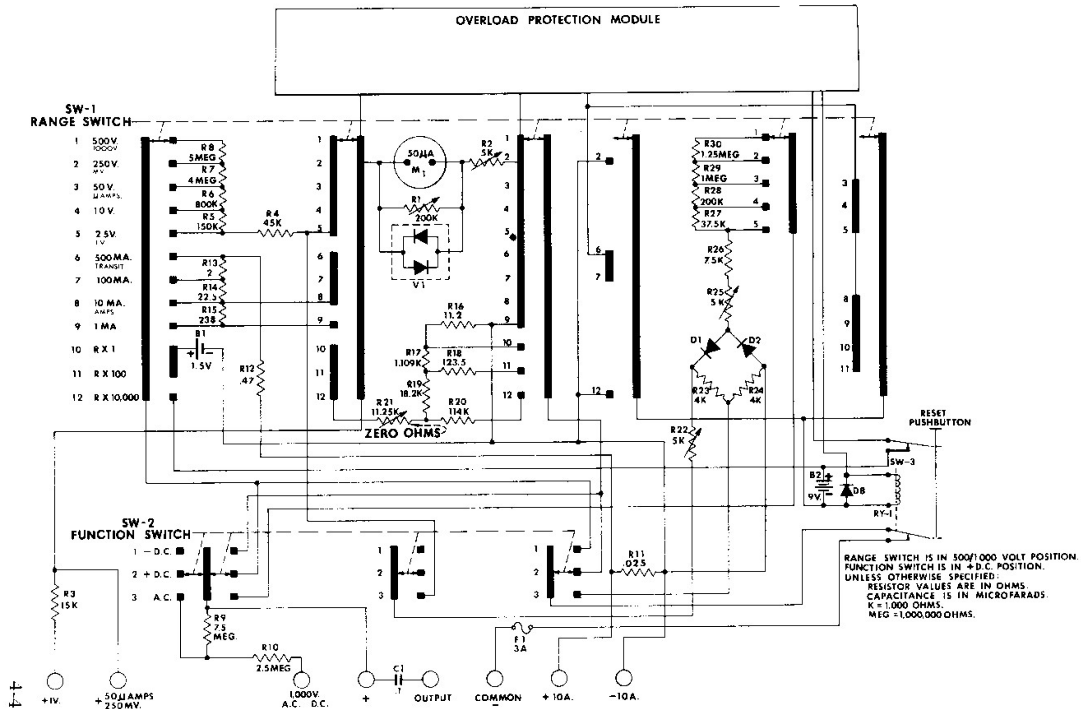
Figure 4-1. Simpson 260-6P, Schematic Diagram
