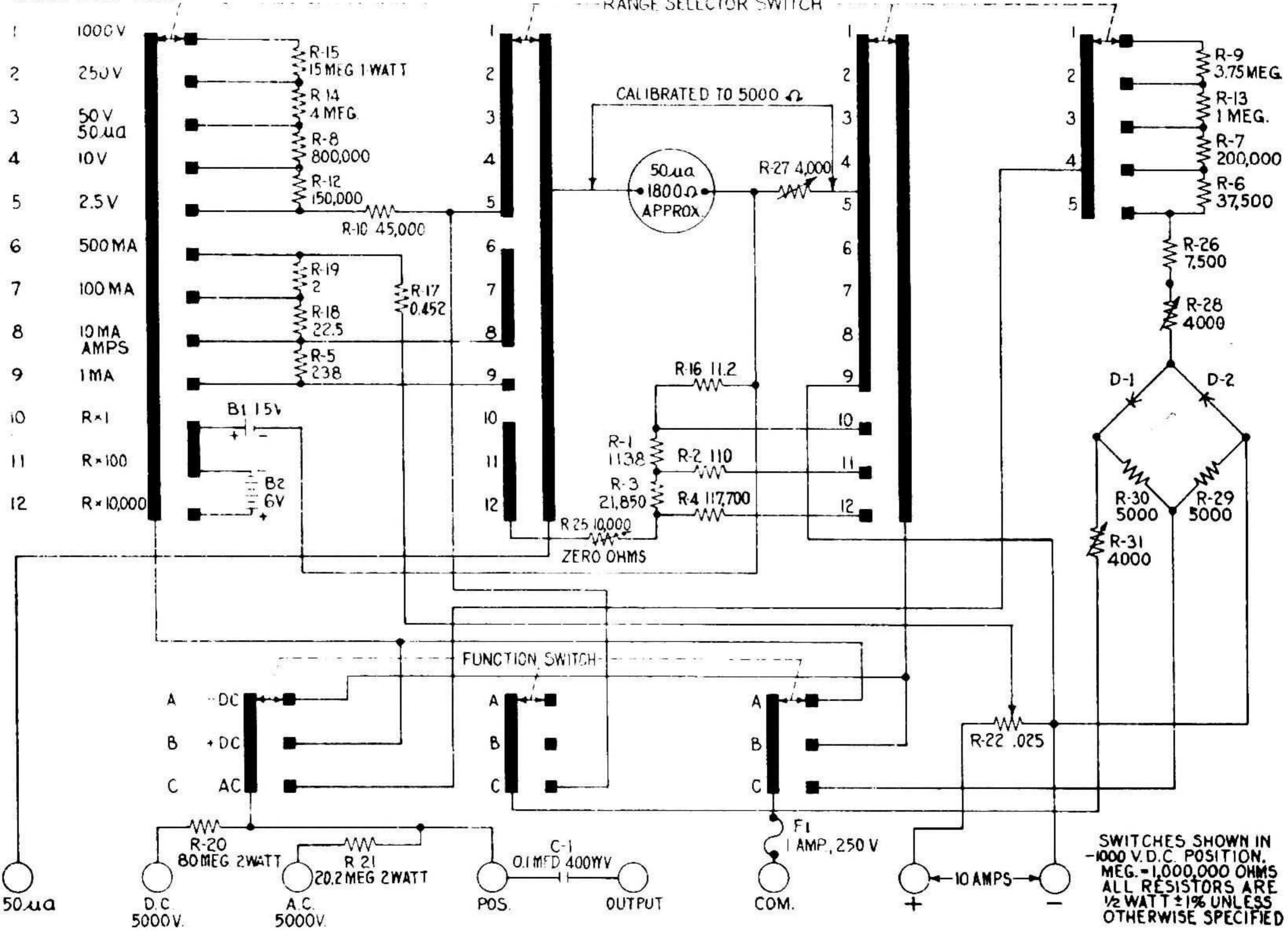
FIGURE 2. OVERALL SCHEMATIC, SIMPSON VOLT-OHM-MILLIAMMETER 260 ® SERIES III
