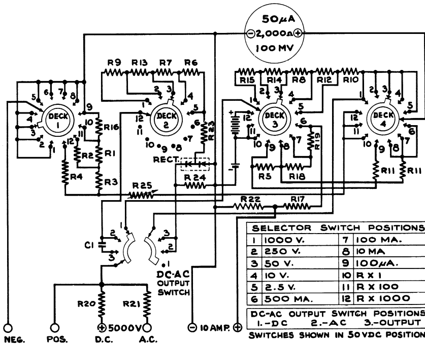
FIGURE 9. MODEL 260 SCHEMATIC DIAGRAM
