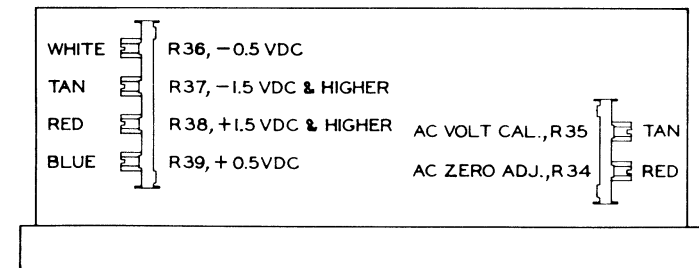
FIGURE 2. LOCATIONS OF CALIBRATING CONTROLS
